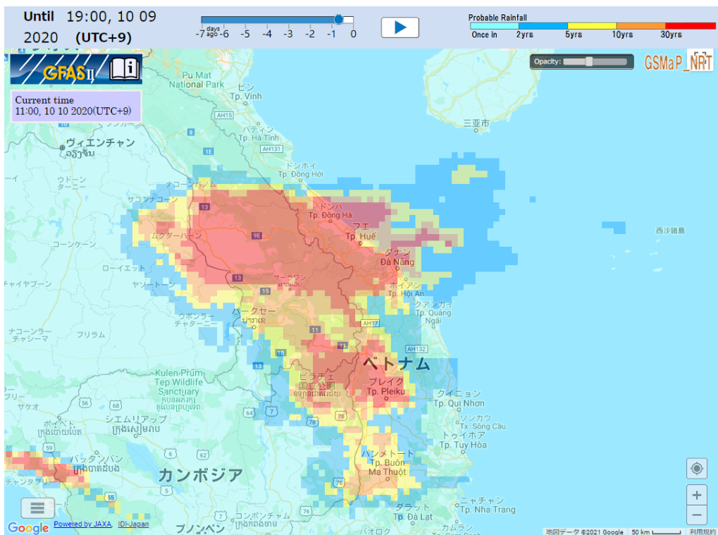
72h Probable Rainfall (7:00pm, Oct. 6 to 7:00pm, Oct. 9 JST)
