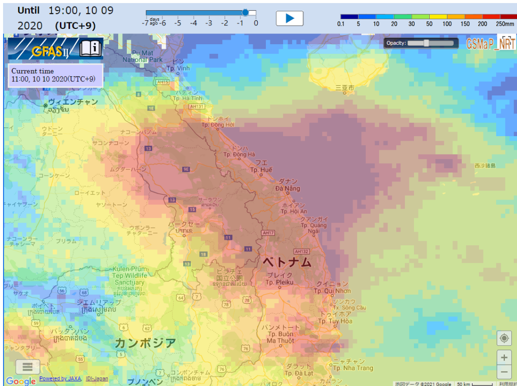
72h Accumulated Rainfall (7:00pm, Oct. 6 to 7:00pm, Oct. 9 JST)
